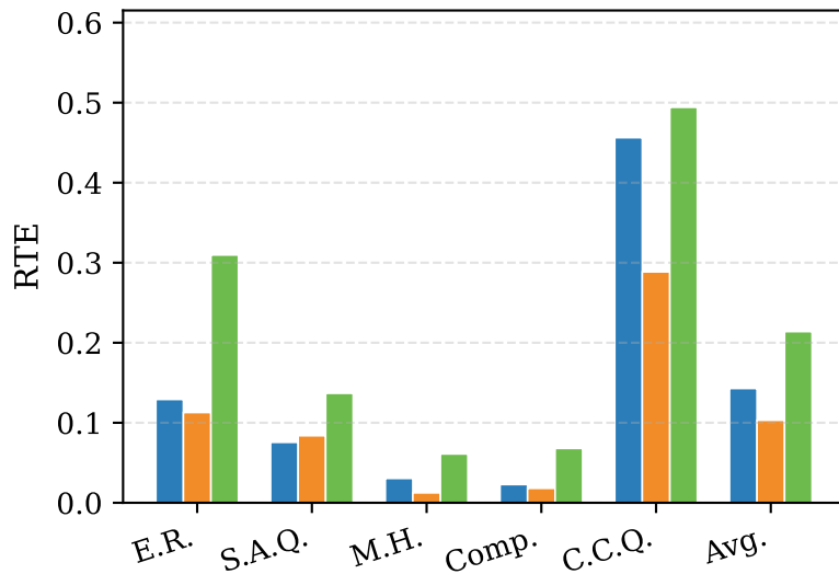
InternVL3.5-8B
