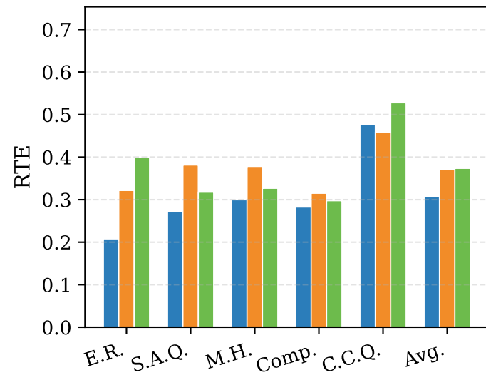
Qwen2.5-vl-7B
