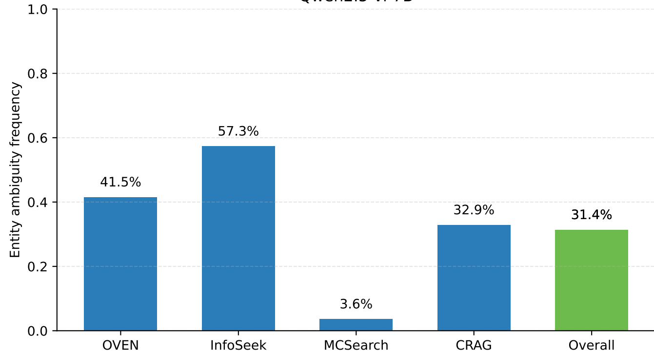
Qwen2.5-vl-7B
