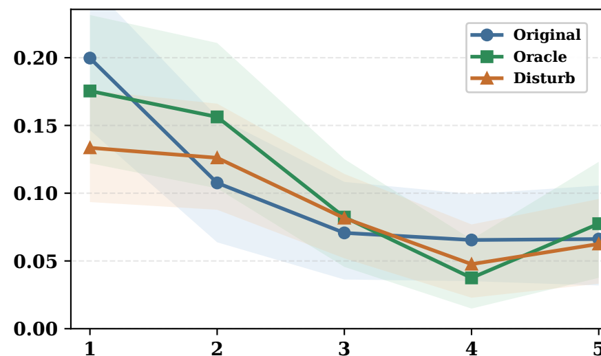
InternVL3.5-8B
