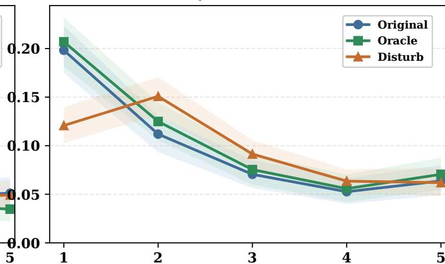
InternVL3.5-8B
