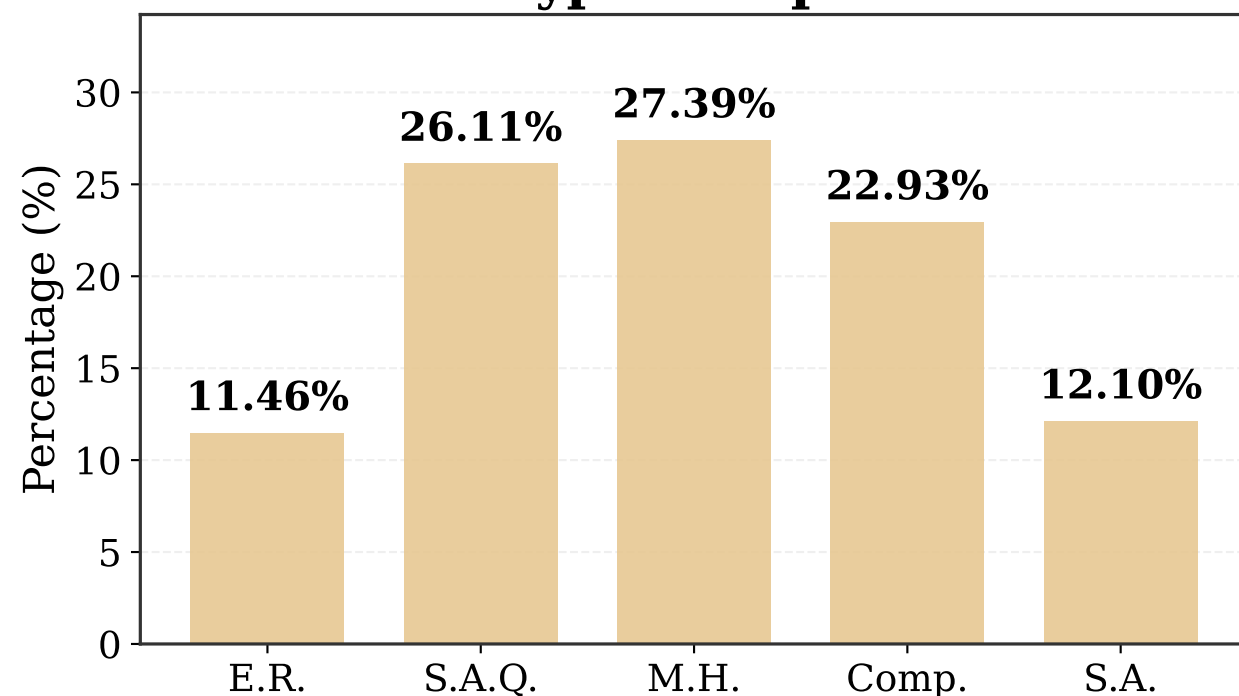
Task-type Composition
