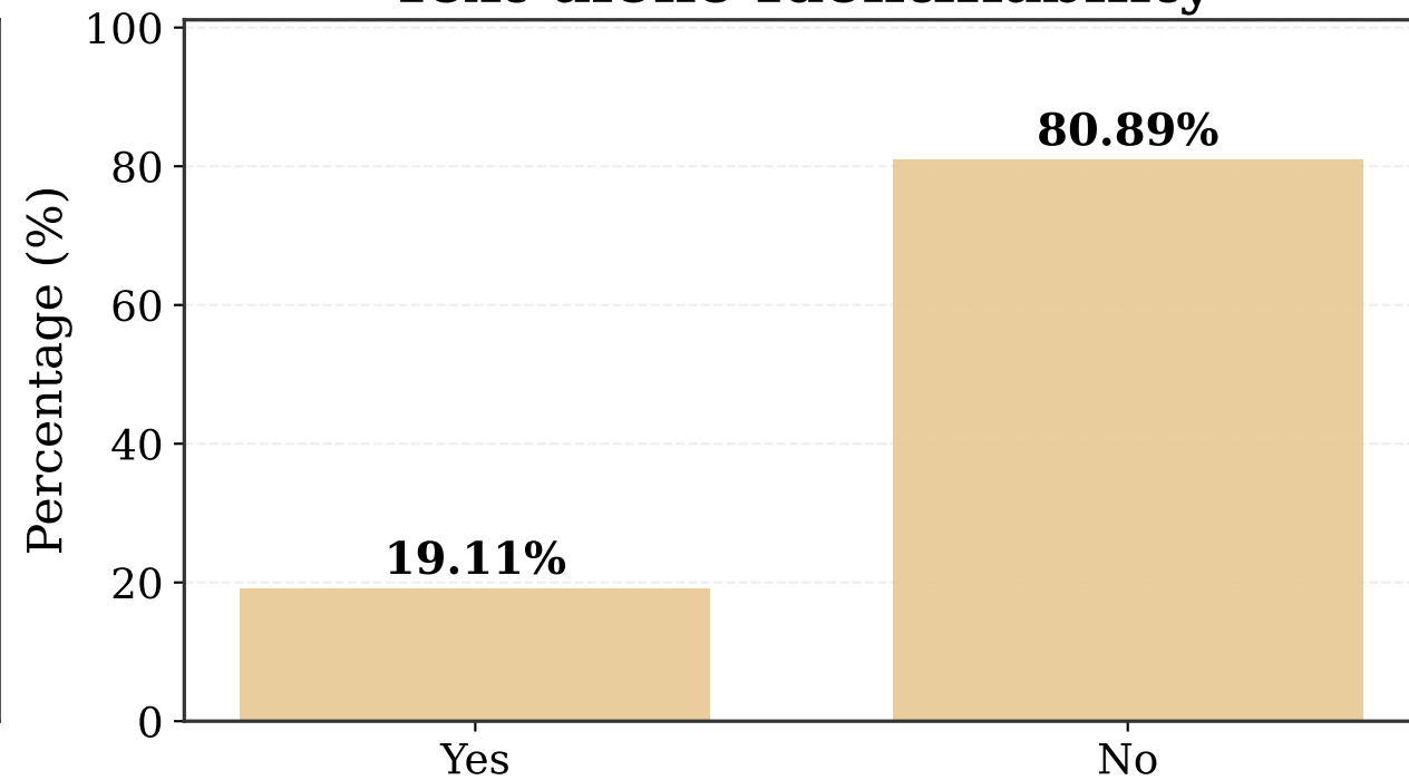
Text-alone Identifiability
