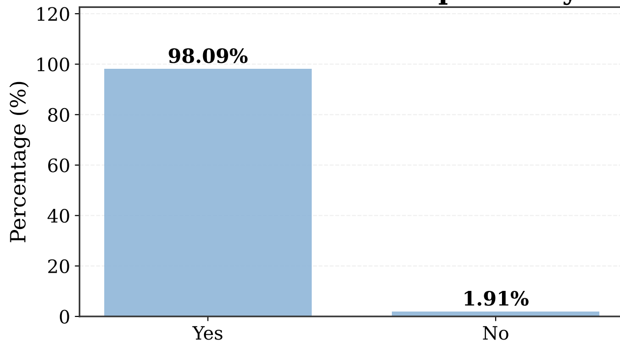
External-evidence Dependency
