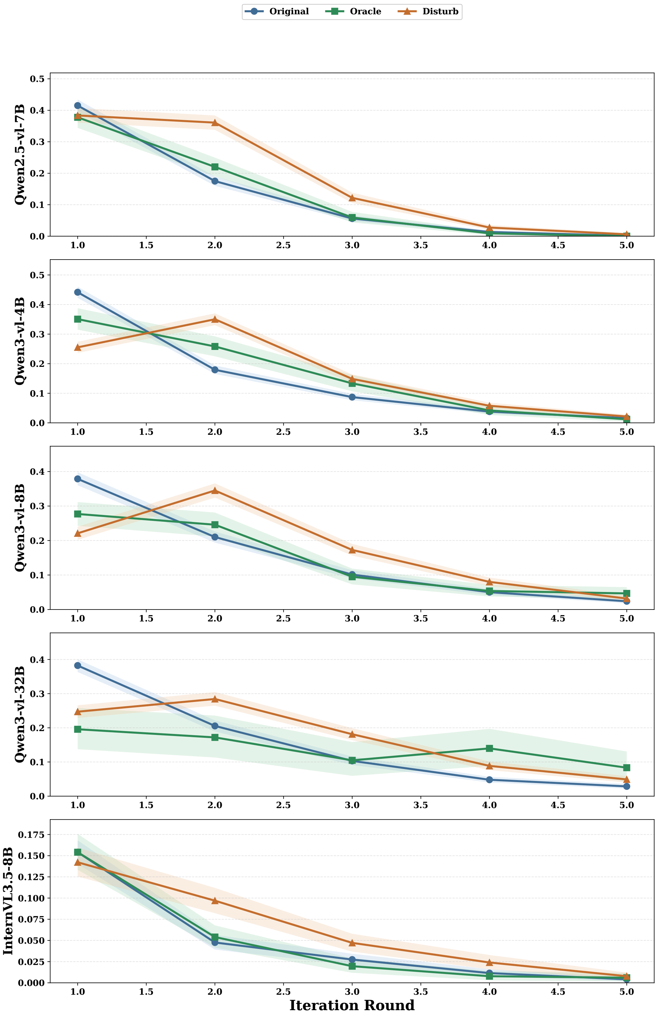
Trajectory-level step-score decay (zero-padded after termination)
