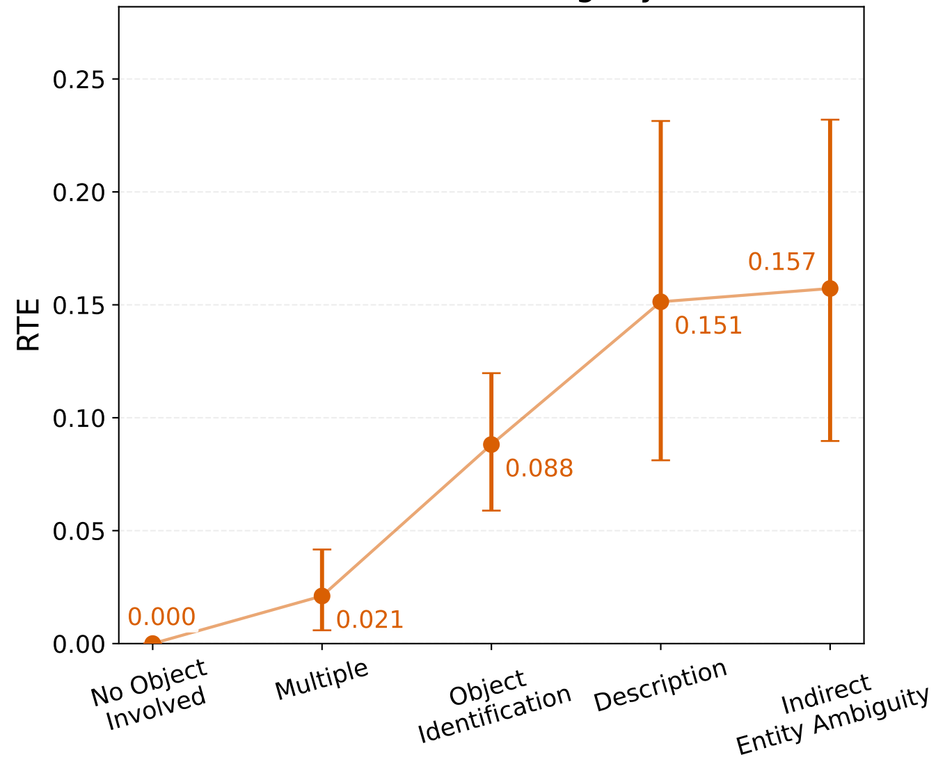
(b) Fine-Grained Ambiguity Levels
