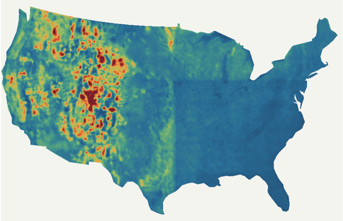
Figure 1: Example FireWx-FM active-fire occupancy heatmap generated from 2026-07-06 12:00 UTC HRRR input, with a 12-hour lead to 2026-07-07 00:00 UTC. Brighter colors indicate higher predicted active-fire occupancy probability. The rendered image is percentile-scaled for visualization; quantitative analysis should use the probability raster.
