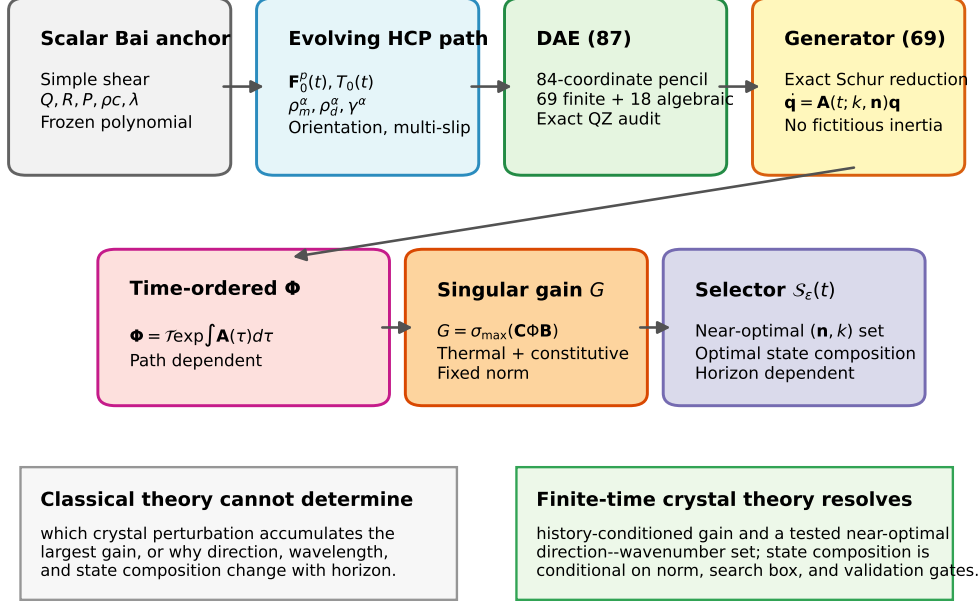
Figure 1: Theory and variable framework. The classical scalar Bai problem provides the instantaneous thermoplastic anchor; the HCP formulation resolves orientation, 18 slip systems, dislocation populations, temperature, inertia and algebraic micromorphic fields; exact descriptor reduction then permits time-ordered finite-time selection. The strict analytical HCP-to-Bai limit remains an explicit open gate.
