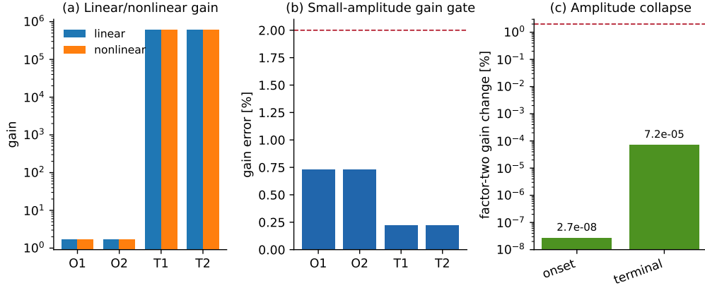
Figure 10: Four-mode Galerkin transport check for the actual near-onset and terminal optimal inputs; O1/O2 and T1/T2 denote the two factor-two amplitudes at onset and terminal horizons. (a) Linear and nonlinear gains. (b) Relative gain errors remain below the preregistered 2% gate within this subspace. (c) Factor-two gain changes are orders of magnitude below the 2% amplitude-collapse gate. The separate dealiased full-grid audit converges in resolved gain but fails the discarded-right-hand-side-energy gate, preventing interpretation as complete nonlinear validation.
