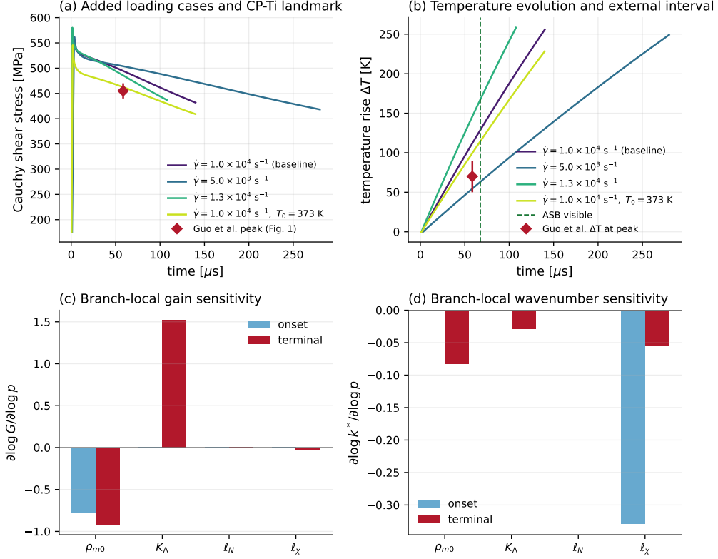
Figure 8: Transfer and validation boundaries. (a,b) Stress and temperature histories for the three added rate/temperature paths, with synchronized Grade-II CP-Ti landmarks from Guo et al. (c,d) Branch-local logarithmic sensitivities of gain and optimized wavenumber to \pm 20\% changes in two dislocation and two gradient parameters. Experimental markers are external timing/scale checks, not fitted data.
