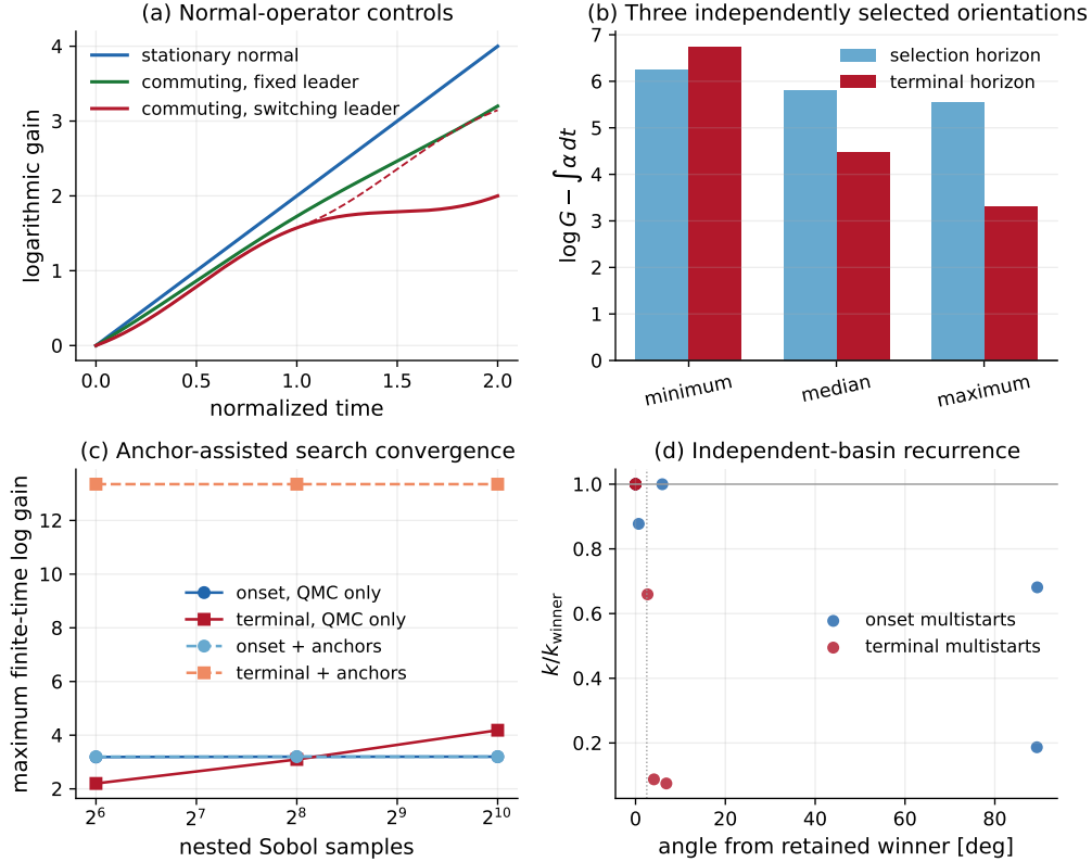
Figure 5: Strengthening audits. (a) Stationary-normal and commuting-normal fixed-leader controls give coincident propagated and frozen-integral curves; a commuting-normal switching-leader control correctly separates them. (b) Like-for-like full-state discrepancies for three independently selected crystal orientations. (c) Nested projective-sphere- \log k reconnaissance, with blind Sobol and anchor-combined maxima shown separately. (d) Recurrence of eight independent local refinements around the retained onset and terminal basins. Panels (c,d) constitute an anchor-assisted basin-retention audit, not a global-optimum certificate.
