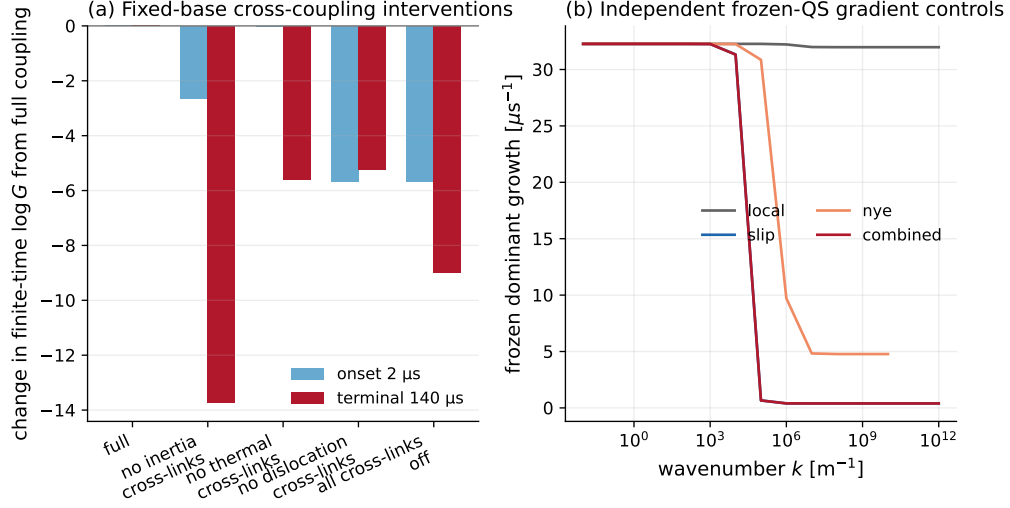
Figure 9: Counterfactual controls. (a) Change in finite-time log gain after grouped removal of cross-coupling blocks while holding the base history and all within-group blocks fixed. The dependence on inertia, thermal and dislocation cross-links changes sharply between 2 and 140 \mu\text{s} . (b) Independent frozen quasi-static gradient audit: full-rank slip-gradient recovery controls the sampled high- k branch, whereas the rank-deficient Nye term alone gives only partial suppression. The panels have separate evidence contracts and are not compared quantitatively.
