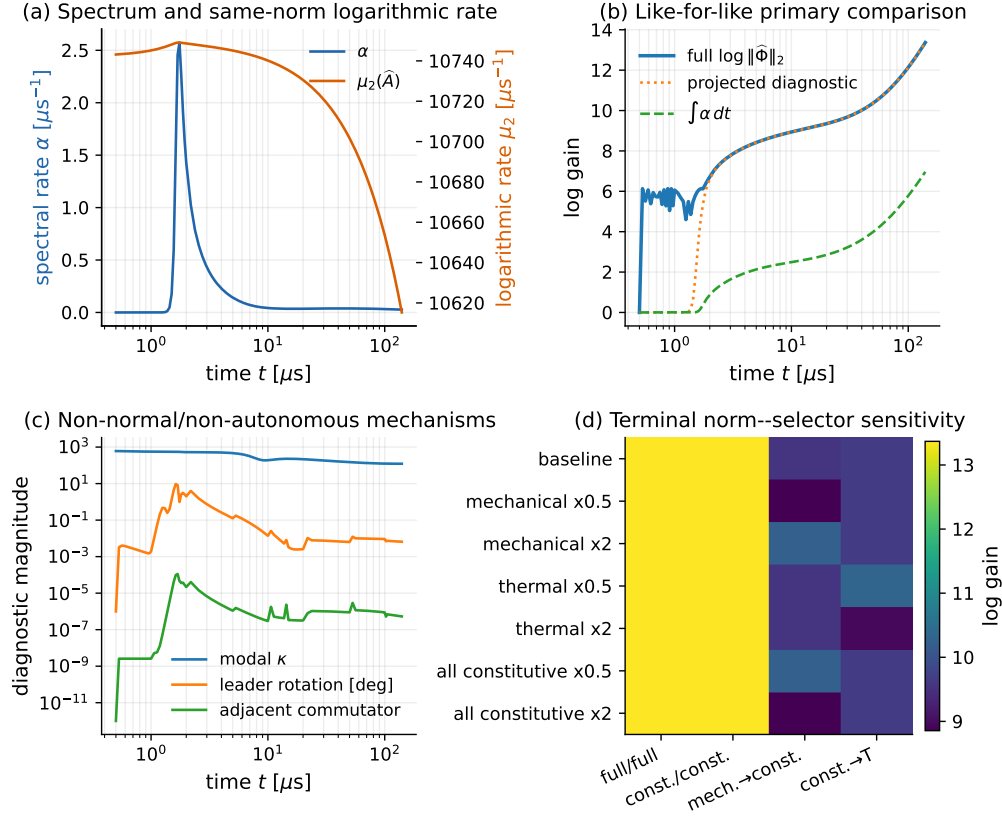
Figure 4: Like-for-like operator and sensitivity audit. (a) Full-state spectral and logarithmic rates for the terminal branch; the latter is a valid but loose same-norm upper bound. (b) Full-state propagator gain and frozen integral on the same 69-state space; the projected constitutive gain is shown separately. (c) Instantaneous leading-mode condition number, adjacent eigenvector rotation and normalized commutator. (d) Terminal gains under representative norm-selector changes; the complete 11-by-7 fixed-candidate matrix is supplied as Supplementary Fig. S1.
