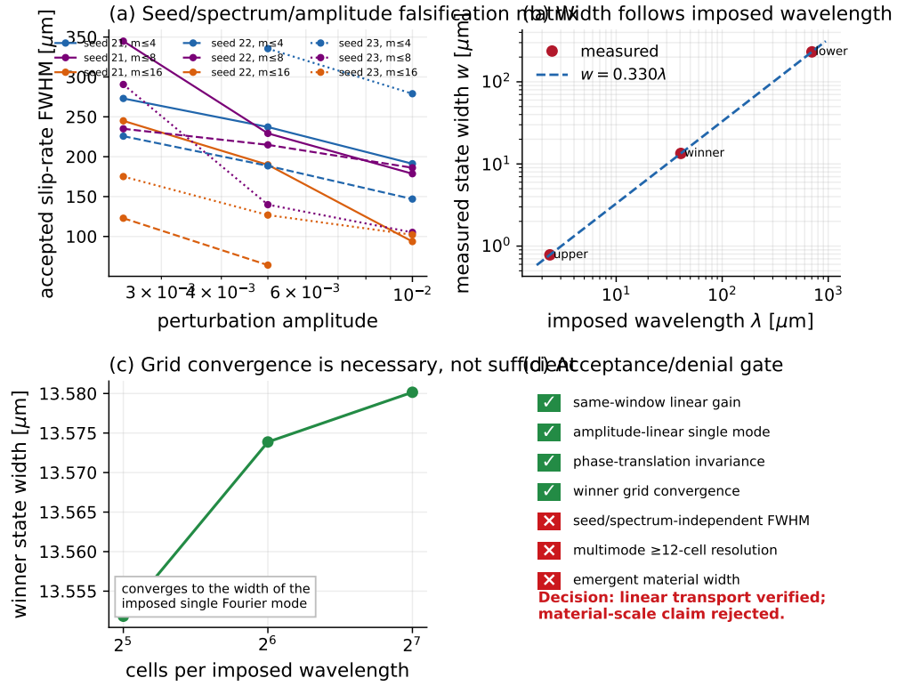
Figure 11: Same-window linear–nonlinear acceptance/denial gate. (a) The FWHM depends on perturbation amplitude, seed and spectral support. (b) Single-mode width follows W \simeq 0.330\lambda_{\text{input}} . (c) That imposed-mode width converges under grid refinement. (d) Gain, amplitude linearity, phase translation and winner-grid convergence pass, whereas seed-independent FWHM, 12-cell multimode resolution and an emergent material width fail.
