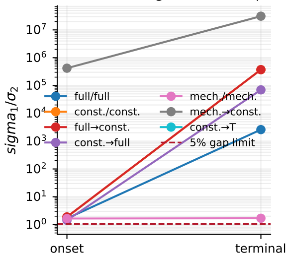
(c) Formal singular-value separation
