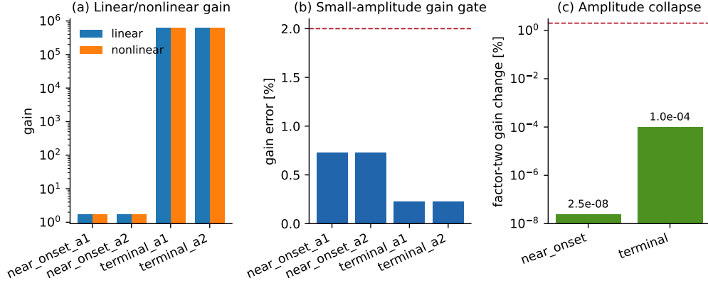
Figure 10: Four-mode Galerkin transport check for the actual near-onset and terminal optimal inputs. (a) Linear and nonlinear gains for two factor-two amplitudes at each horizon. (b) Relative gain errors remain below the preregistered 2% gate within this subspace. (c) Factor-two gain changes are orders of magnitude below the 2% amplitude-collapse gate. The separate full-Fourier audit remains open and prevents interpreting this figure as complete nonlinear validation.
