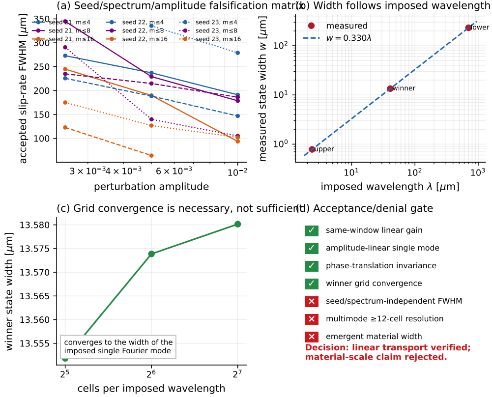
Figure 11: Same-window linear-nonlinear acceptance/denial gate. (a) The FWHM depends on perturbation amplitude, seed and spectral support. (b) Single-mode width follows W \simeq 0.330\lambda_{\text{input}} . (c) That imposed-mode width converges under grid refinement. (d) Gain, amplitude linearity, phase translation and winner-grid convergence pass, whereas seed-independent FWHM, 12-cell multimode resolution and an emergent material width fail.
