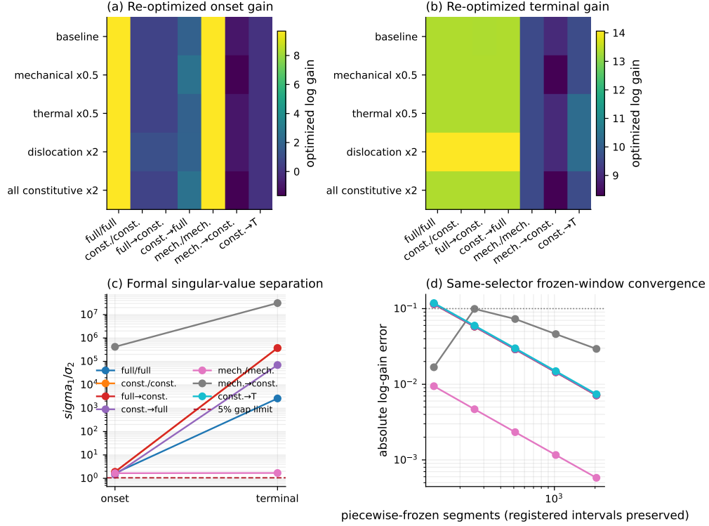
Figure 7: Selector-specific direction–wavenumber re-optimization. (a,b) Optimized log gains for seven selectors under the baseline and four adverse norms. (c) Onset and terminal singular-value ratios with the formal 5% relative-gap threshold; rank-one temperature outputs are not assigned a ratio. (d) Convergence of the same- \mathbf{P}_{\text{in}}/\mathbf{P}_{\text{out}} piecewise-frozen propagator while preserving every registered nonuniform base-state interval. Boundary k maxima are classified as wave branches and are not converted into localization wavelengths.
