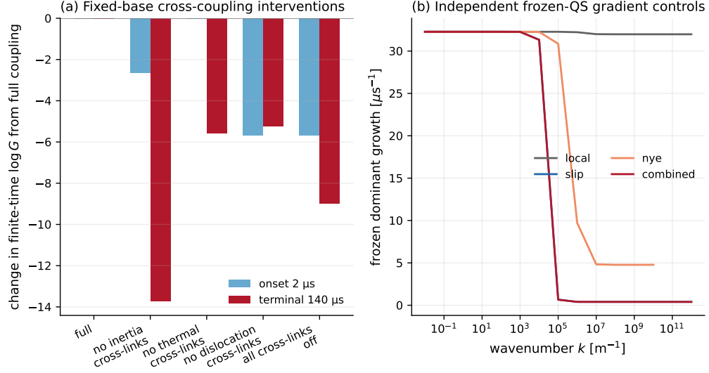
Figure 9: Counterfactual controls. (a) Change in finite-time log gain after grouped removal of cross-coupling blocks while holding the base history and all within-group blocks fixed. The dependence on inertia, thermal and dislocation cross-links changes sharply between 2 and 140 \mu s. (b) Independent frozen quasi-static gradient audit: full-rank slip-gradient recovery controls the sampled high- k branch, whereas the rank-deficient Nye term alone gives only partial suppression. The panels have separate evidence contracts and are not compared quantitatively.
