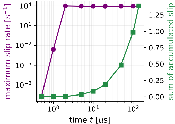
(b) Slip-system activation
