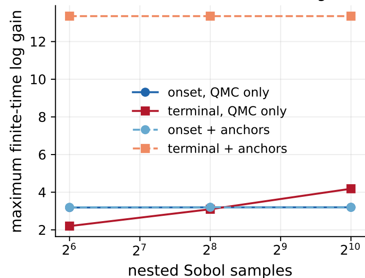
(c) Anchor-assisted search convergence
