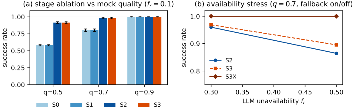
Figure 9: Architectural ablation (mock LLM, seeded, 150 tasks \times 3 seeds). (a) Success rate by pipeline stage and injected quality. (b) Availability stress isolating the fallback layer (narrow vs. full template coverage: S3 vs. S3X).
