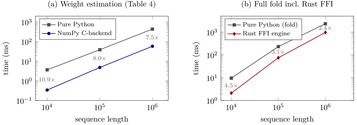
Figure 3: System-level acceleration of the Unibit pipeline (log-log). (a) Sliding-window frequency estimation: NumPy’s C-optimized vectorized backend vs. pure Python (7.5x–10.9x). (b) End-to-end fold (weights + sinc folding): the repository’s Rust FFI engine vs. pure Python (4.5x–2.4x, including Python-side normalization and marshaling overhead; Table 5).
