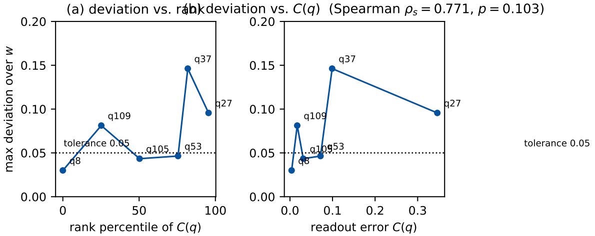
Figure 8: C(q) -guided routing validation. (a) Maximum measured deviation vs. the score’s rank percentile: the top-ranked qubits pass, but deviations are not monotone along the ranking (q109 at percentile 25.2% already exceeds tolerance), so no upper-half rule is validated at this n . (b) Deviation vs. raw readout error C(q) (Spearman \rho_s = 0.771 , exact permutation p = 0.103 , n=6 ). Data: analysis/results/router_analysis.json .
