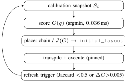
Fig. 1. The UniMind scheduling loop. One scoring pass is sub-millisecond; the refresh trigger decides when the stored snapshot must be re-fetched. (execution \rightarrow results) is emitted downstream.
