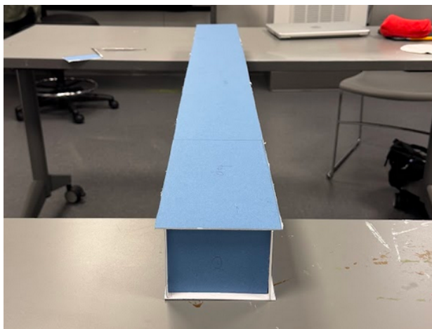
FIG. 7. Bridge as of the end of day on Nov 20th. 9:00 PM, Nov 20.
