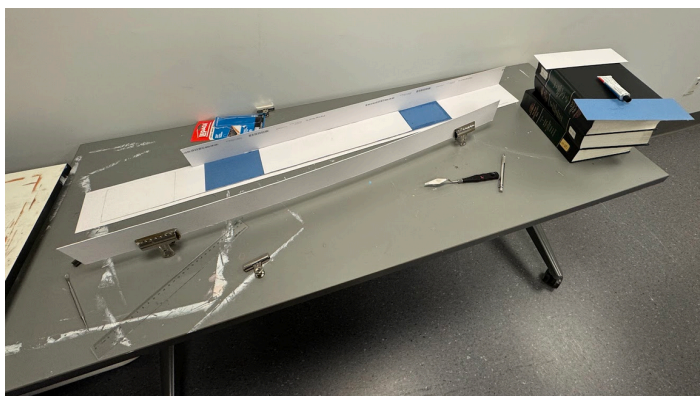
FIG. 4. Gluing the web. The web was glued following the tracks. 5:00 PM, Nov 20.
