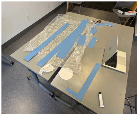
Figure 9: Keeping the main table clean. We placed a tarp here even though these pieces of matboard were not dirty.
