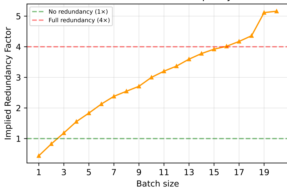
Traffic Model / DRAM Capacity
