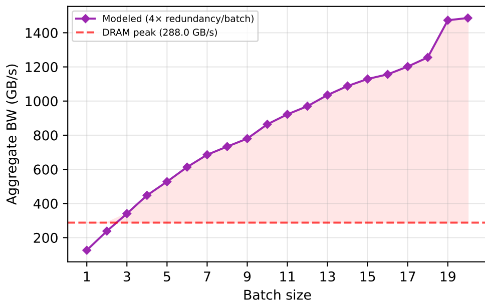
Modeled DRAM BW Demand
