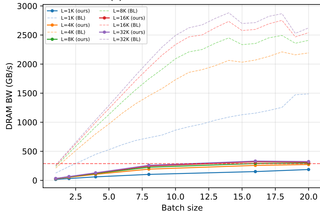
(c) Effective DRAM Bandwidth
