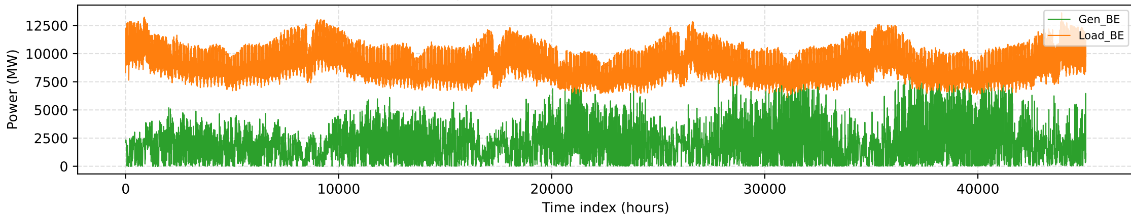
Belgium Renewable Generation and Load (MW)
