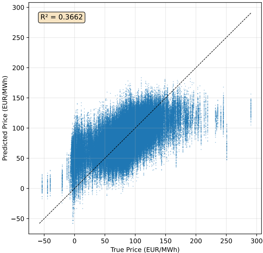
ForecastModel: True vs Predicted on Test Set
