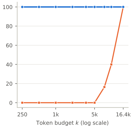
(e) Rare concepts (<100 events) represented (%) \uparrow
