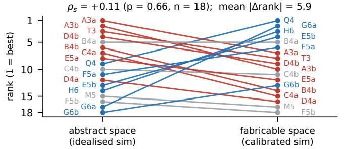
Fig. 1. Flat-ground ranking of the 18 morphologies in the abstract (left) and fabricable (right) space. Blue lines rise, red lines fall, grey lines move at most 2 ranks. Q4/T3/M5/H6: hand-designed quadruped, tripod, mixed, hexapod; A–G: the seven DoF-partition species, two generation-0 samples (a, b) each; the digit is the leg count.
