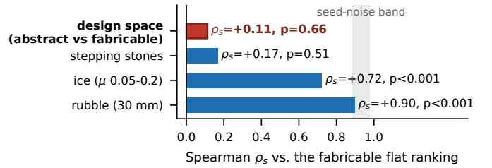
Fig. 2. Spearman rank correlation of each ranking with the fabricable flat-ground ranking. Shaded: the 5–95% range that seed noise alone produces at the median measured CV.
