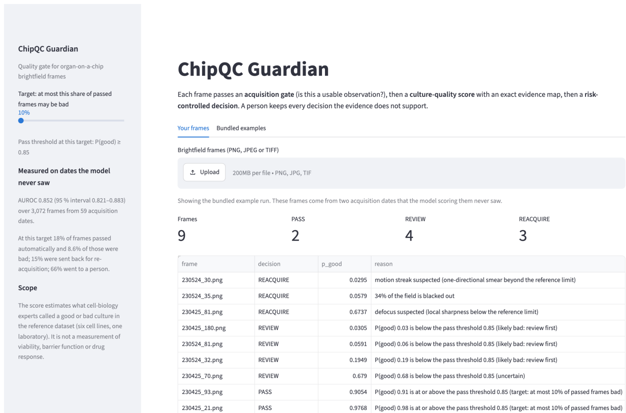
Figure 4. The review console on the bundled example run: outcome counts, the ordered audit table and, below it, one card per frame with the frame, its evidence map, the acquisition descriptors and similar reference frames.
