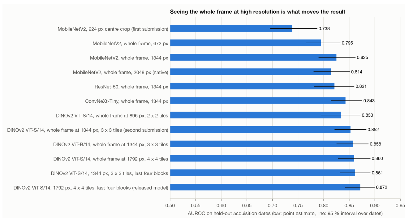
Figure 6. AUROC on held-out dates for each representation, with 95 % intervals over dates.
