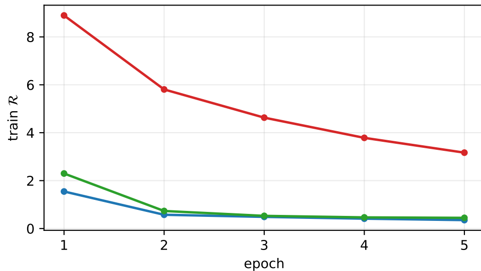
Signal 3%: adjacent-subjet \mathcal{R}
