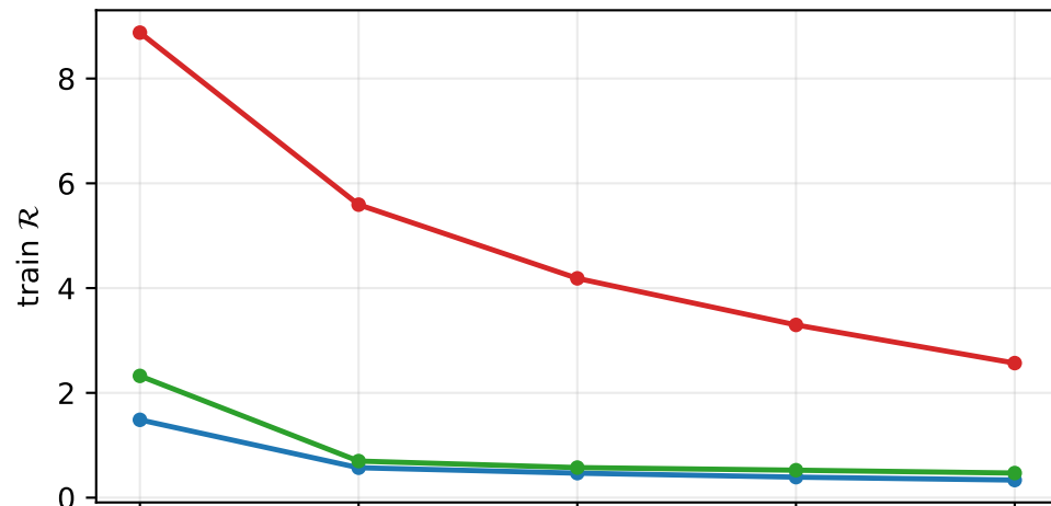
Signal 0%: adjacent-subjet \mathcal{R}
