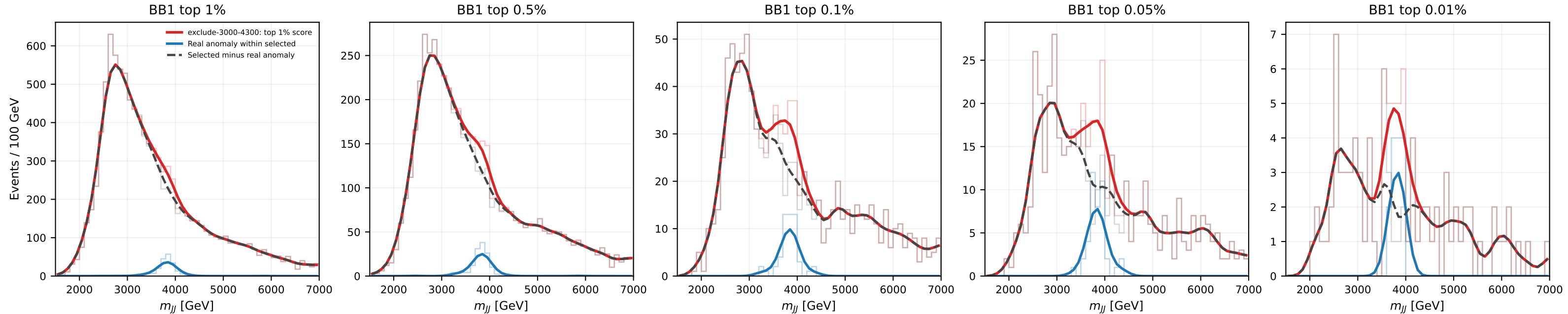
BB1 exclude 3000 \leq m_{jj} < 4300 : top-score selection with truth decomposition (last.pt)
