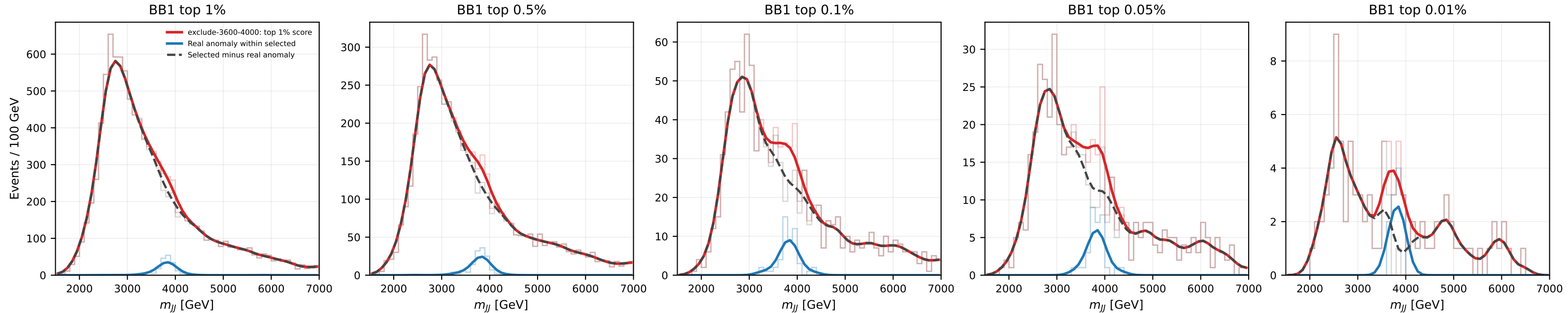
BB1 exclude 3600 \leq m_{jj} < 4000 : top-score selection with truth decomposition (last.pt)
