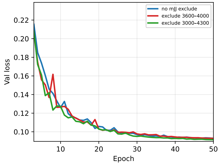
Val loss (epoch \geq 3 )
