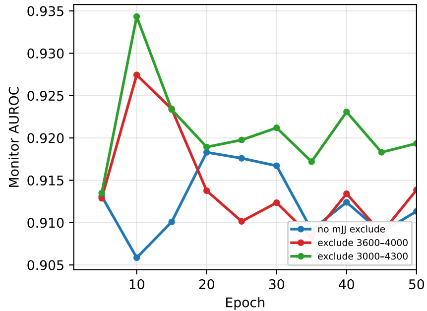
Monitor AUROC (diagnostic)
