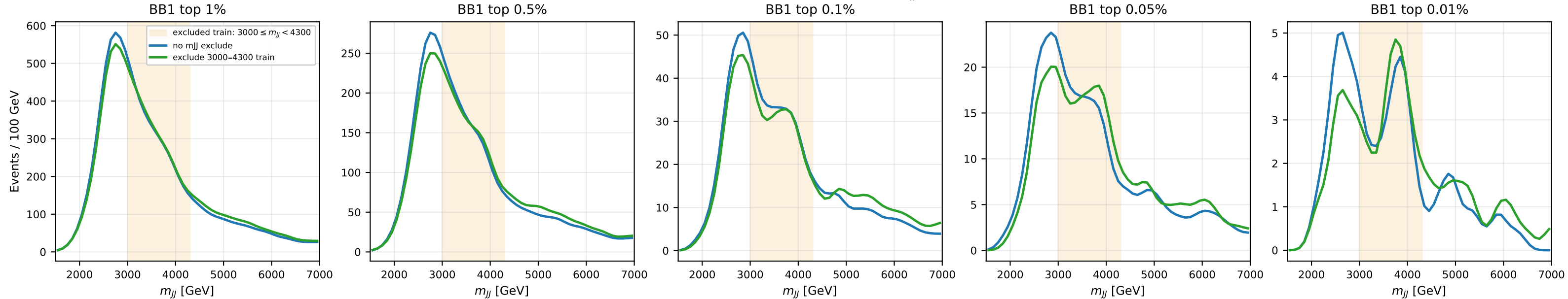
BB1 top selection: no-exclude vs exclude 3000 \leq m_{jj} < 4300 (last.pt)
