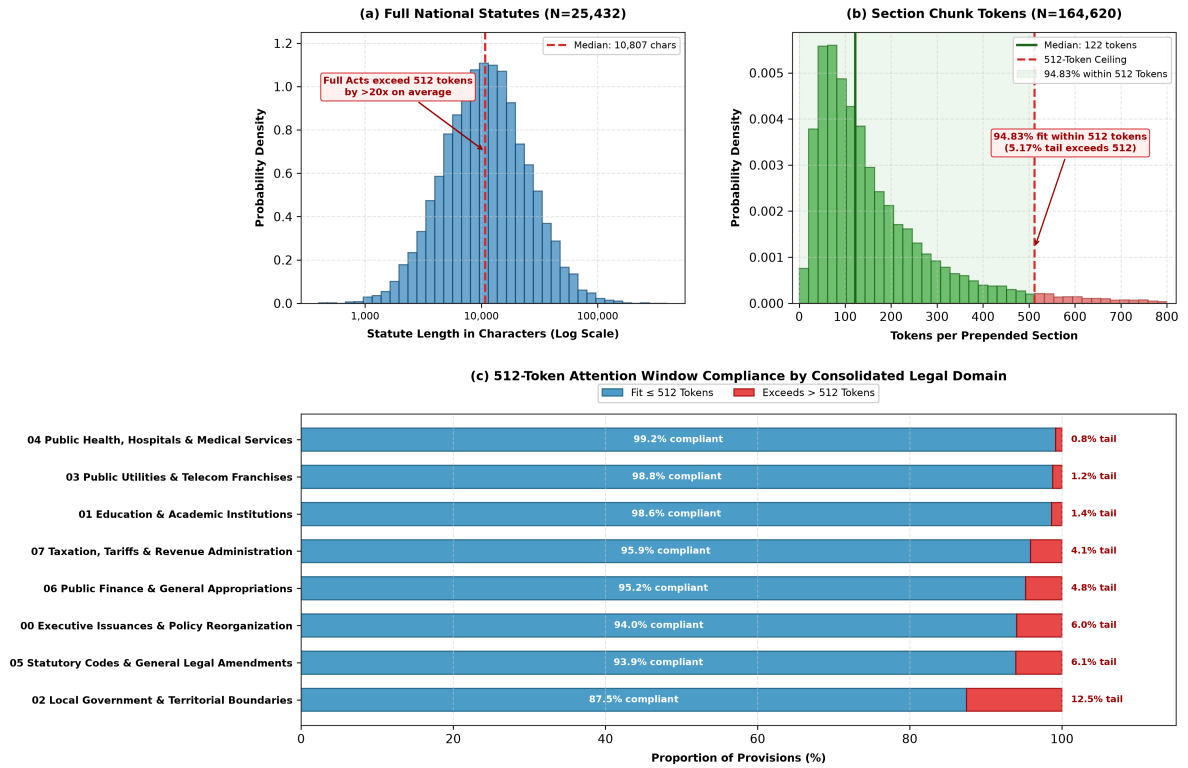
Figure 3.8: Document Length Distributions, Prepend Section Token Granularity, and 512-Token Compliance Rates across the Philippine National Statutory Corpus ( N = 25,432 Statutes, N = 164,620 Sections).
