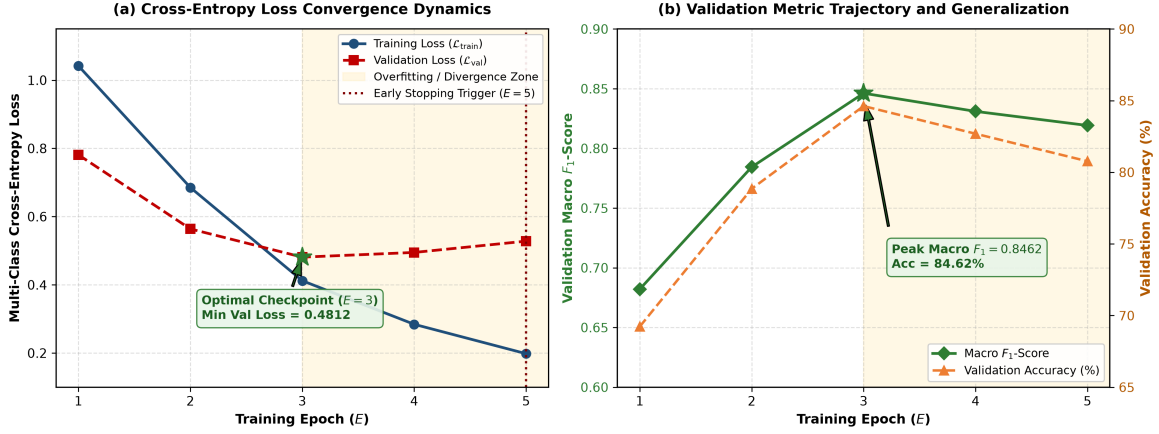
Figure 4.2: Stage 2 Cross-Encoder Loss Dynamics and Convergence Trajectory across Fine-Tuning Epochs ( \eta = 2 \times 10^{-5} , B = 8 ). Panel A traces the training loss against validation holdout loss, illustrating the optimal bias-variance inflection point at Epoch 3 and the subsequent early stopping divergence. Panel B tracks the corresponding validation accuracy and Macro F_1 -score progression.
