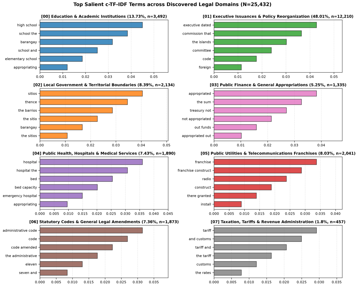
Figure 3.6: Top Salient c -TF-IDF Keyword Profiles across the Eight Consolidated Macro Legal Domains ( N = 25,432 ).
