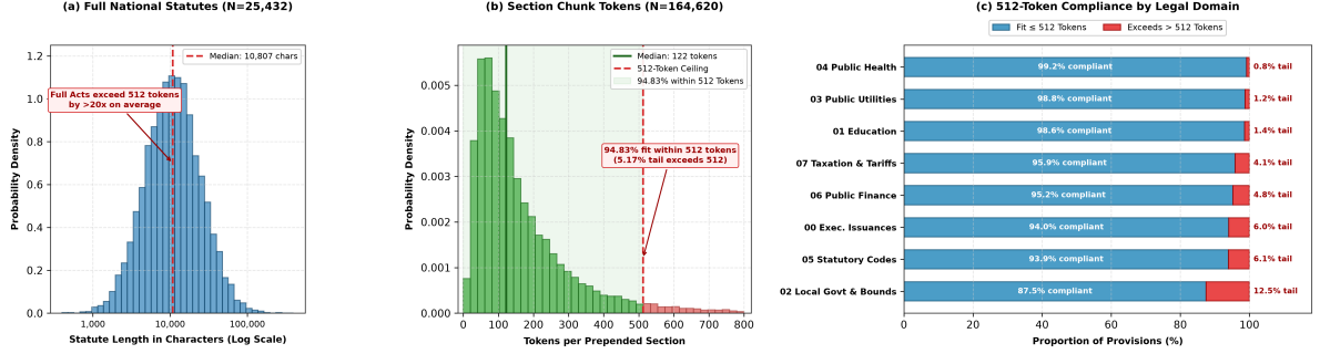
Figure 3.8: Document Length Distributions, Prepended Section Token Granularity, and 512-Token Compliance Rates across the Philippine National Statutory Corpus ( N = 25,432 Statutes, N = 164,620 Sections).
