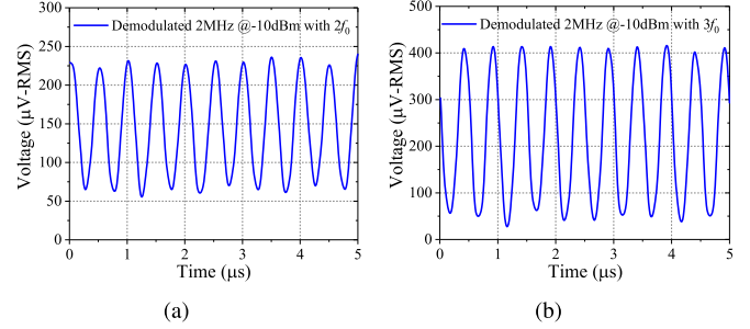
Fig. 9. Demodulated 2 MHz square-wave from (a) 2f_0 carrier and (b) 3f_0 carrier; the spectrum analyzer is set to zero-frequency span mode, the Y-axis is in linear scale and its unit is root-mean-square (RMS) value in volts.
