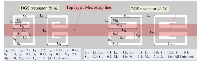
Fig. 5. Physical dimensions of the DGS resonators used in the reconfigurable BSF.
