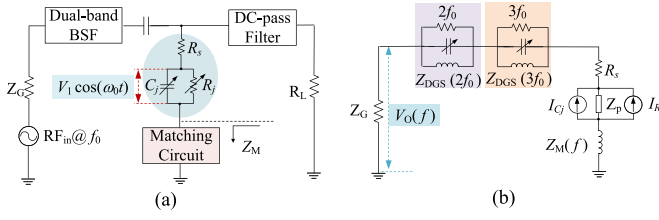
Fig. 2. (a) Block diagram of the proposed HBR. (b) Equivalent circuits describing the proposed HBR at harmonic frequencies.
