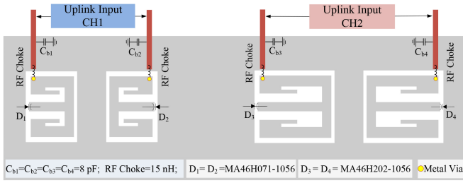
Fig. 6. Bottom view of the reconfigurable BSF with varactors and bias circuits.
