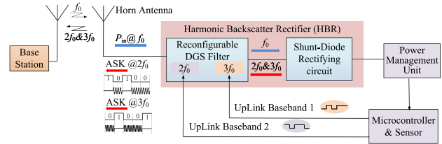
Fig. 1. System illustration of the proposed harmonic backscatter rectifier, where the reradiated harmonics can be modulated in amplitude through a dual-band reconfigurable band-stop filter using DGS.
