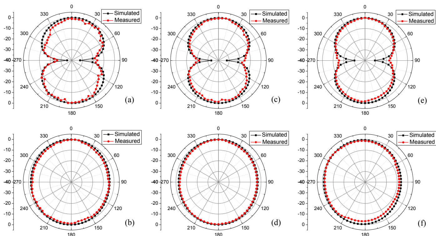
Fig. 7 Simulated and measured radiation patterns: (a) yz -plane at 3.85 GHz; (b) xz -plane at 3.85 GHz; (c) yz -plane at 4.5 GHz; (d) xz -plane at 4.5 GHz; (e) yz -plane at 6.5 GHz; (f) xz -plane at 6.5 GHz;
