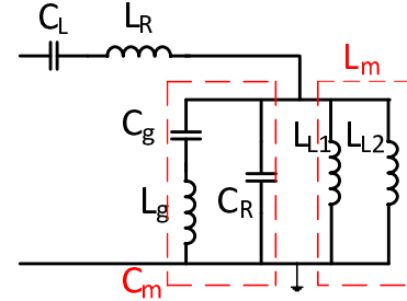
Fig. 4 The equivalent circuit of the proposed antenna.
