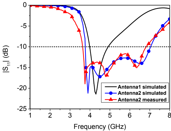
Fig. 5 Comparison of S_{11} between the two antennas.
