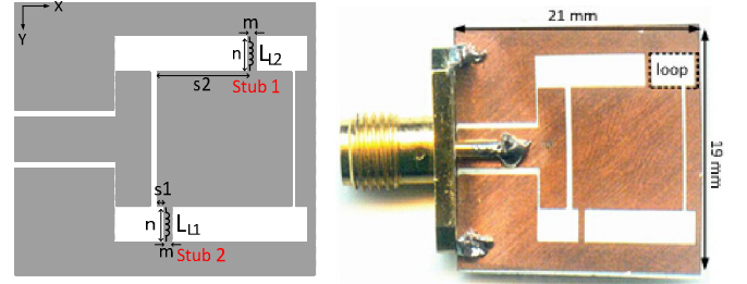
Fig. 3 (a) Geometry of the antenna. (b) Fabricated prototype of the antenna.
