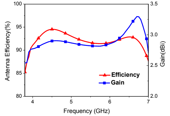
Fig. 6 Simulated gain and efficiency of the antenna
