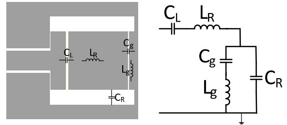
Fig.1. Equivalent circuit of the proposed antenna.
