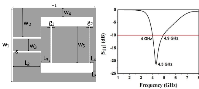
Fig. 2 (a) Dimensions. (b) Simulated return loss.
