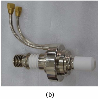
Fig. 1. (a) The diagram of two injection-locked magnetrons applied to microwave power combining system; (b) The 15 kW magnetron
