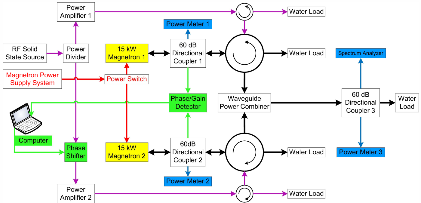
Fig. 2. The block diagram of two way injection-locked 15 kW CW magnetrons microwave power combining system.
