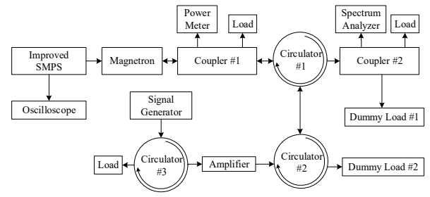
Fig. 3. Diagram of the experiment system.
