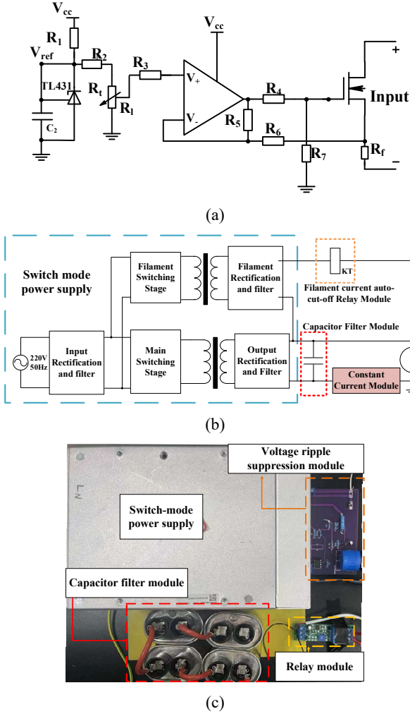
Fig. 2. (a) Diagram of the designed CRE. (b) Structure diagram of the switch-mode power supply. (c) Photograph of the switch-mode power supply.
