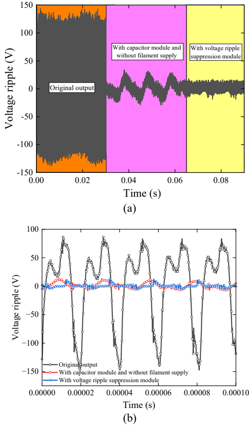
Fig. 4. Anode voltage ripple of the magnetron. (a) Total ripples. (b) High frequency ripples.
