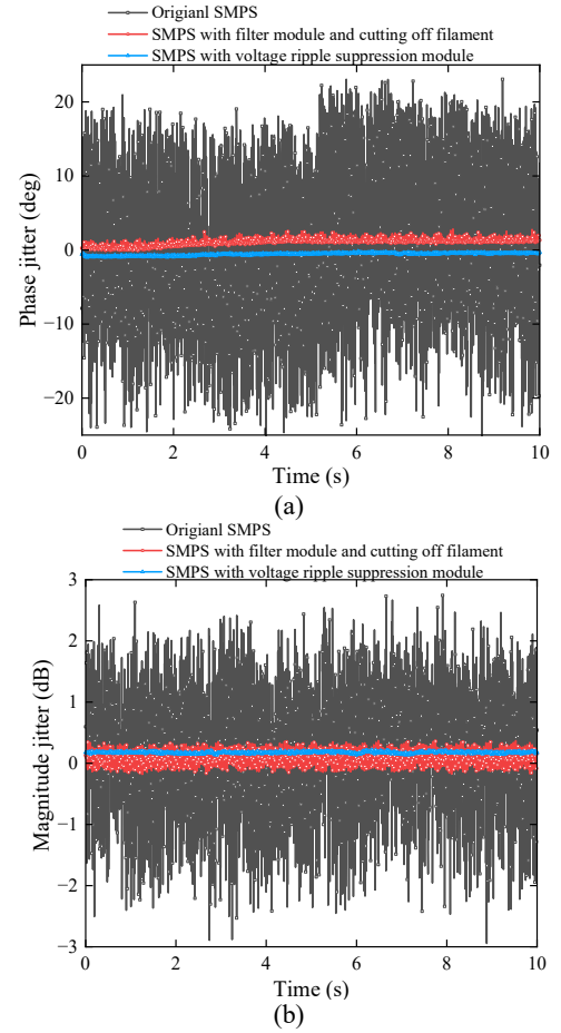
Fig. 5. Output characteristics of the injection-locked magnetron under different conditions. (a) Output phase jitter. (b) Output magnitude jitter.
