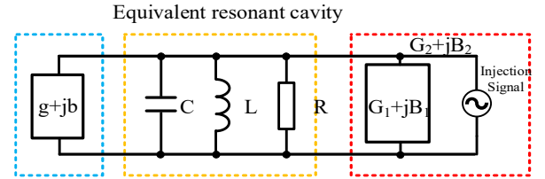
Fig. 1. Equivalent circuits of a magnetron's resonant cavity.
