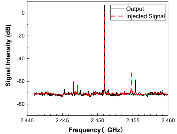
Fig. 4. FM noise suppression in the injection locking operation (RBW: 30Hz, VBW: 30Hz)
