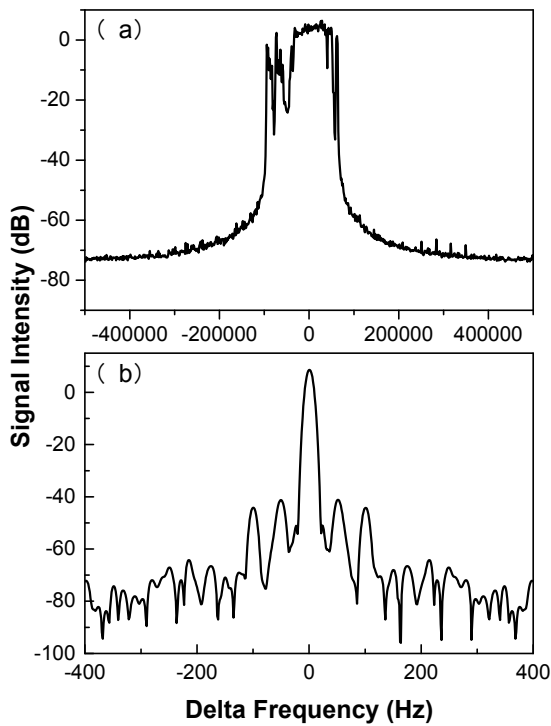
Fig. 3 The oscillation spectrum of magnetron at different states (RBW: 10Hz, VBW: 10Hz)
