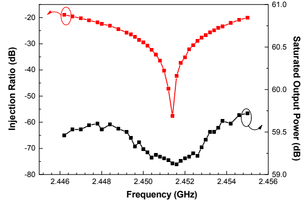
Fig. 2 The minimum injection power ratio and saturated output power at different frequency
