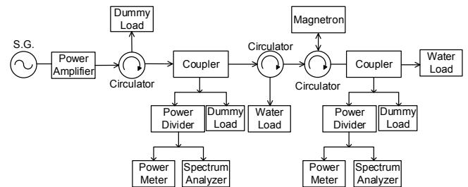
Fig. 1 Block diagram of the low power injection-locked CW magnetron system
