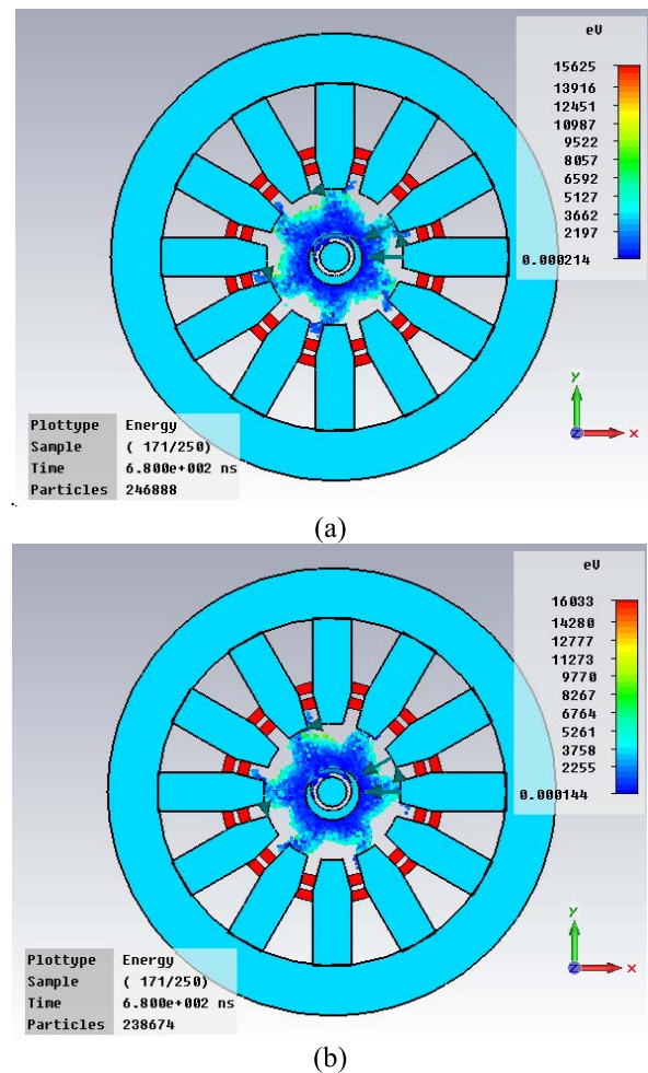
Fig. 15. Electron bunch formation of the injected signals (free-running output is 17.2 kW) for a magnetron injection-locked at (a) 2.450 GHz and (b) 2.451 GHz. The amplitude of the injected signals is constant.
