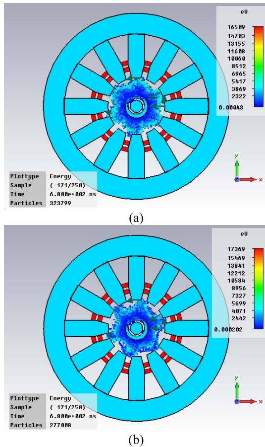
Fig. 12. Electron bunch formation of the injected signals (anode current: \sim 0.7 A). The upper and lower images correspond to the injection-locked magnetron at 2.444 and 2.450 GHz, respectively. The amplitude of the injected signals is constant.
