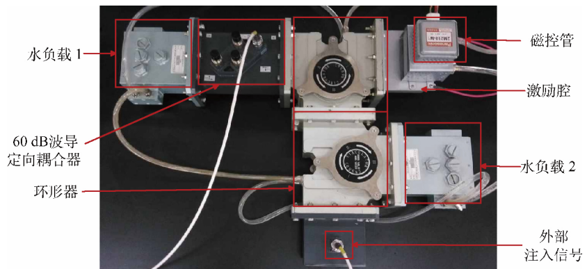
图 3 注入锁频试验系统布局 Fig. 3 Configuration of the inject-locking experimental system
