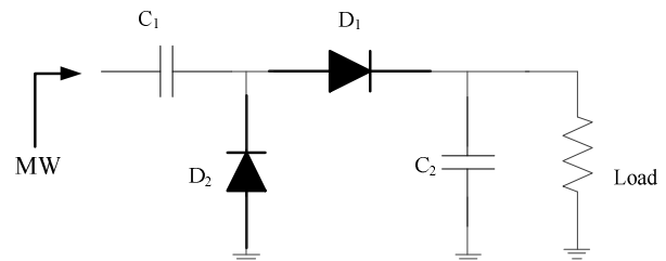
Fig. 1 The model of a voltage doubler rectifier
