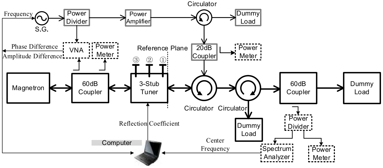
Fig. 2. Diagram of the 1-kW CW magnetron amplifier system (dashed framework part: measurement setup; upper part: injection signal route; Middle highlight path: high-power output route; and connections to computer: control signal route).
