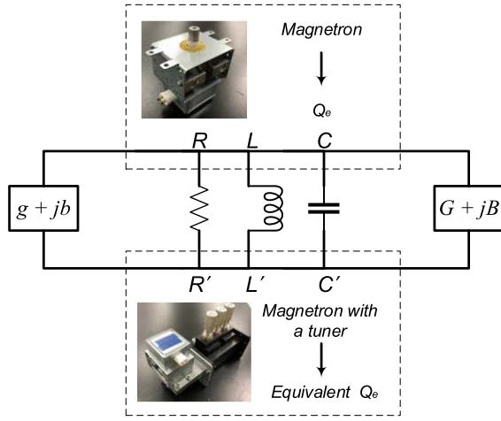
Fig. 1. Equivalent parallel RLC resonance circuit of a magnetron.
