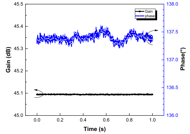
Fig. 7. Amplitude and phase jitter of the magnetron amplifier with a 45-dB power gain.
