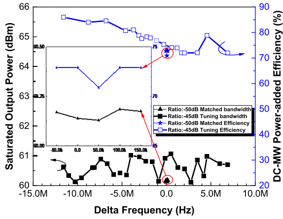
Fig. 6. Output and locked bandwidth of the magnetron amplifier with matched or tuning loads, respectively.
