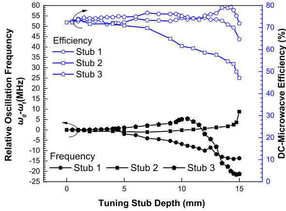
Fig. 4. Frequency and efficiency of free-running magnetron with various tuning stub depths.
