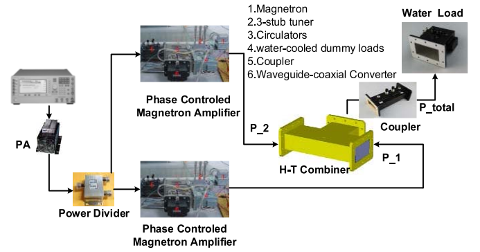
Fig. 9. Diagram of the dual magnetron amplifiers used for microwave power combining.
