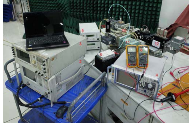
Fig. 5. Hardware setup for the 1-kW CW magnetron amplifier system (1: computer; 2: vector network analyzer; 3: signal generator; 4: signal analyzer; 5: power meter; 6: power amplifier with isolators; 7: high-voltage probe; 8: Fluke multimeter; 9: waveguide-coaxial converter; 10: circulators; 11: water-cooled dummy loads; 12: three-stub tuner; 13: 60-dB coupler; 14: magnetron and external excitation cavity; and 15: 20-dB coupler).
