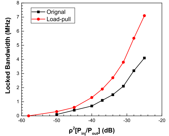
Fig. 3. Injection-Locked bandwidth with various injection ratios at different states.
