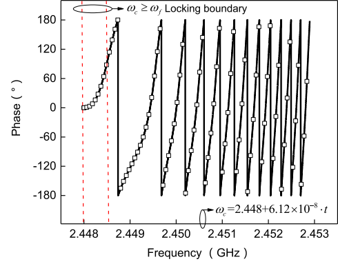
Fig. 2. Output phases in comparison to the coupling frequencies.
