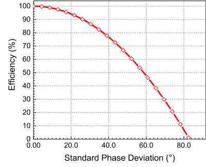
Fig. 1. Power combining efficiency with different standard phase deviations.
