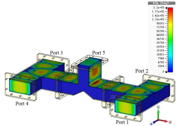
Fig. 6. E-field distribution for the four-way power combining with an incident power of 80 kW.
