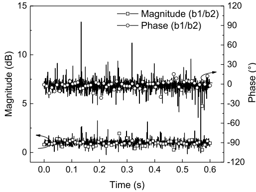
Fig. 7. Amplitude and phase difference of magnetron No. 1 and No. 2 with the above frequency distribution.
