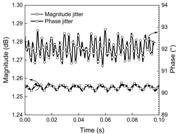
Fig. 9. Relative amplitude and phase jitters of the total output.
