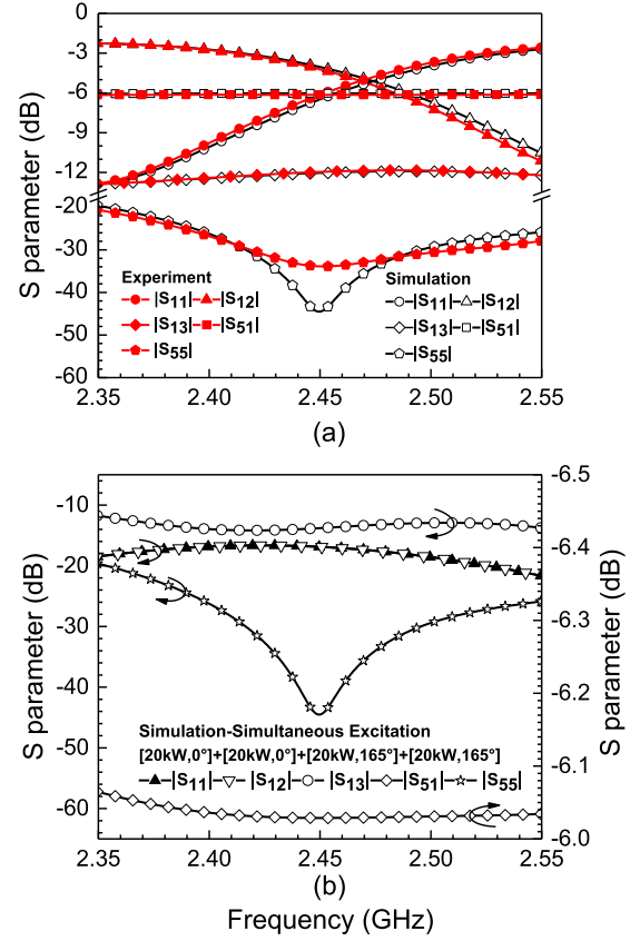
Fig. 5. (a) Simulated and experimental S-parameter of the five-port power combiner. (b) Simulated S-parameter of the desired input amplitudes and phases.
