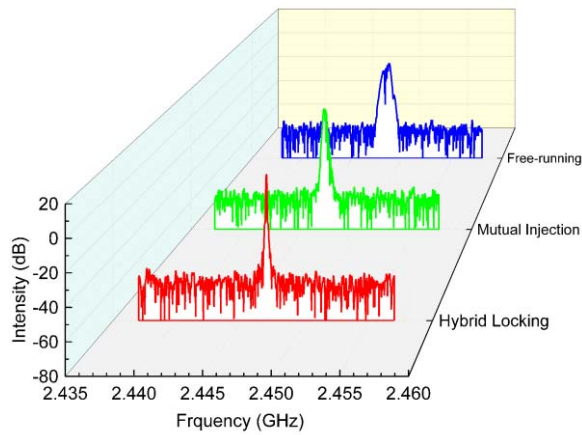
Fig. 8. Spectra of the magnetron's output in different states (RBW of 50 kHz and VBW of 50 kHz).
