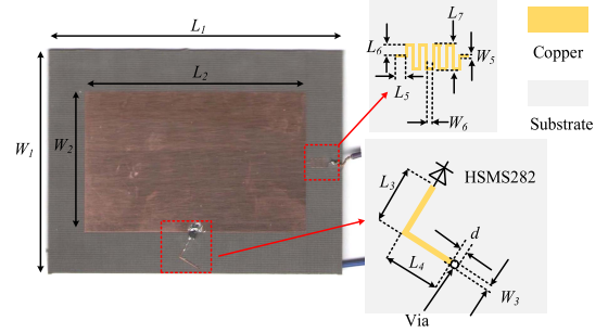
Fig. 7. Fabricated rectangular patch rectenna.
