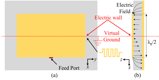
Fig. 6. (a) Topology and (b) electric field distribution of the patch antenna.
