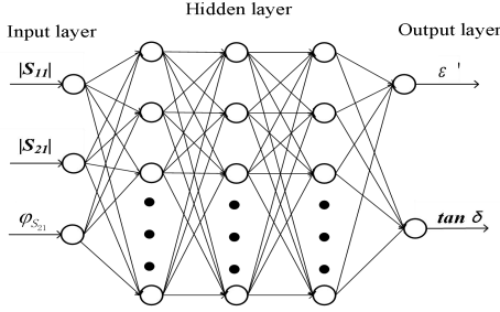
Figure 4. Neural network model.
