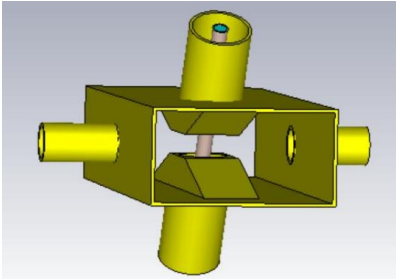
Figure 2. Schematic of oblique aperture ridge waveguide.
