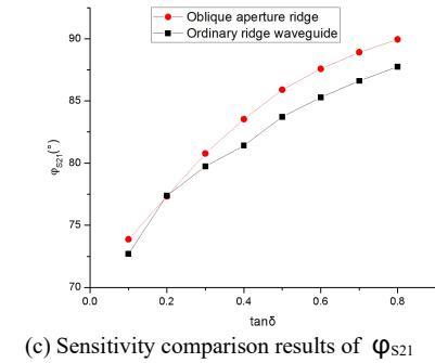
Figure 3. Sensitivity comparison results of ordinary ridge waveguide and oblique aperture ridge waveguide at 2.45GHz.
