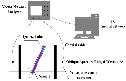
Figure 1. Schematic diagram of measuring system.
