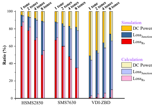
Fig. 6. Simulated and calculated results, including the losses produced by the diodes and the dc-output, at -20 dBm, for different number of tones and diodes.
