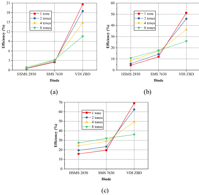
Fig. 4. Simulated RF-to-dc conversion efficiency for three different diodes and different number of tones at (a) -30dBm, (b) -20dBm and (c) -10dBm.
