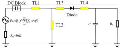
Fig. 1. Circuit schematic of the exploited series-configuration rectifier.
