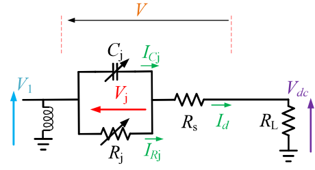
Fig. 5. Nonlinear diode circuit model exploited in the numerical analysis.
