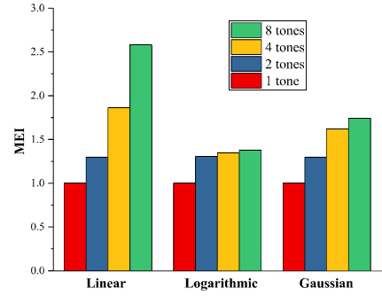
Fig. 3. Simulated MEI values, for -20 dBm at the input port of the HSMS2850 rectifier, for three multitone excitation with up to 8 tones.
