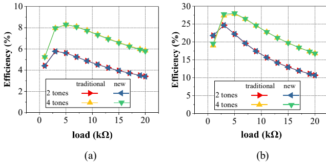
Fig. 2. Comparison of simulated RF-to-dc conversion efficiencies for the HSMS2850 diode at (a) -20 dBm and (b) -10 dBm as function of the load, using the standard multi-tone Harmonic Balance simulation and the method in [8].
