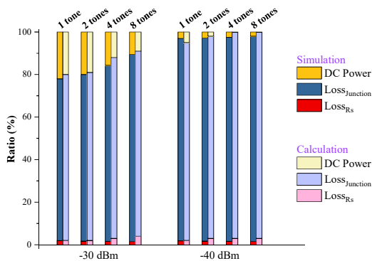
Fig.7 Simulated and calculated losses and performance for the VDI-ZBD diode for -30 dBm and -40 dBm, exploiting up to 8 tones.
