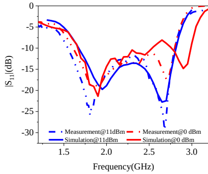
Fig. 8. The reflection coefficient |S_{11}| versus frequency at the input power of 0 dBm and 11 dBm.
