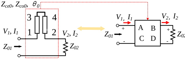
Fig. 2. Schematic diagram of the proposed coupled line and its equivalent two-port network.
