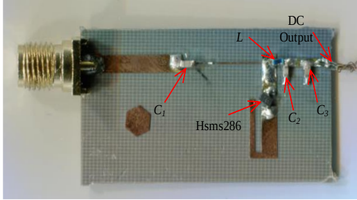
Fig. 7. A photograph of the fabricated rectifier.
