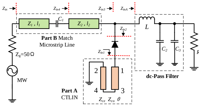
Fig. 1. Proposed rectifier with a wide bandwidth range.
