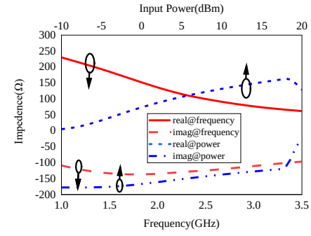
Fig. 3. The variation of Z_d with frequency and input power.
