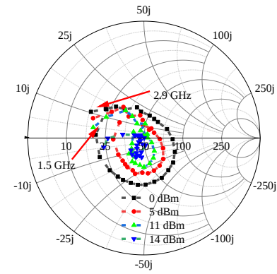
Fig. 5. Z_{in} over 1.5-2.9 GHz at different input power level.
