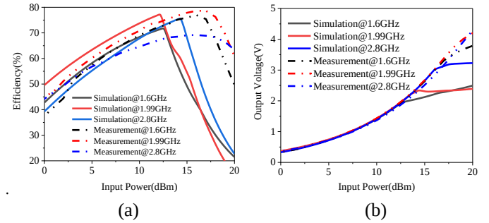
Fig. 11. (a) Conversion efficiency (b) Output Voltage from 0 dBm to 20 dBm at 1.6 GHz, 1.99 GHz, and 2.8 GHz
