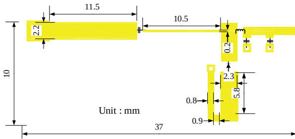
6. Layout of the proposed broadband rectifier.
