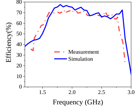
Fig. 10. Measured and simulated RF-dc conversion efficiency versus frequency at the input power of 11 dBm.
