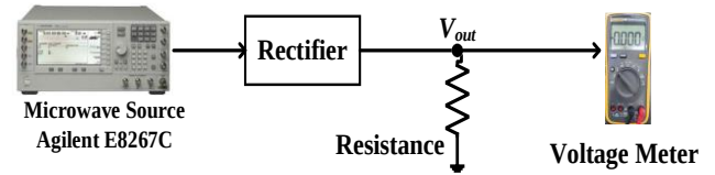
Fig. 9. Diagram of the measurement system.
