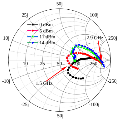
Fig. 4. Z_{in2} over 1.5-2.9 GHz at various input power levels.
