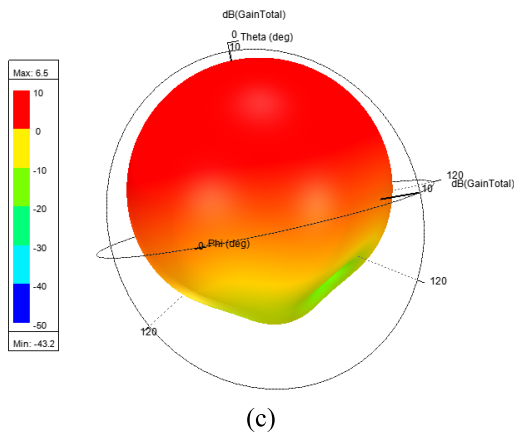
Fig. 6. Simulated radiation patterns at 2.45 GHz. (a) Pattern over the E -plane. (b) Pattern over the H -plane. (c) Three-dimensional pattern.
