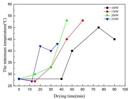
Figure 3. The minimum temperature with time under 100W, 150W, 200W and 250W.
