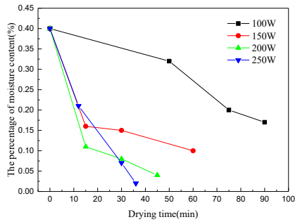
Figure 2. Trend of moisture content with time under 100W, 150W, 200W and 250W.
