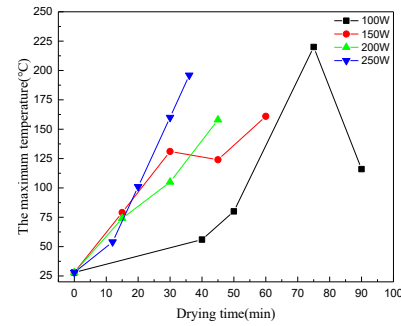
Figure 4. The maximum temperature with time under 100W, 150W, 200W and 250W.
