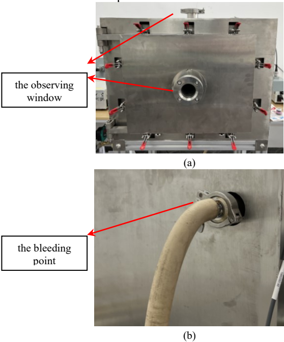
Figure 1. Microwave vacuum deep drying resonant cavity (a)the observe side of cavity(b)the back side of cavity.
