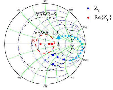
Fig. 3. Diode impedances at different power levels. A: Diode impedance with the imaginary parts. B: Diode impedance without the imaginary parts.
