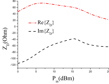
Fig. 2. Diode impedance variations with the input power.
